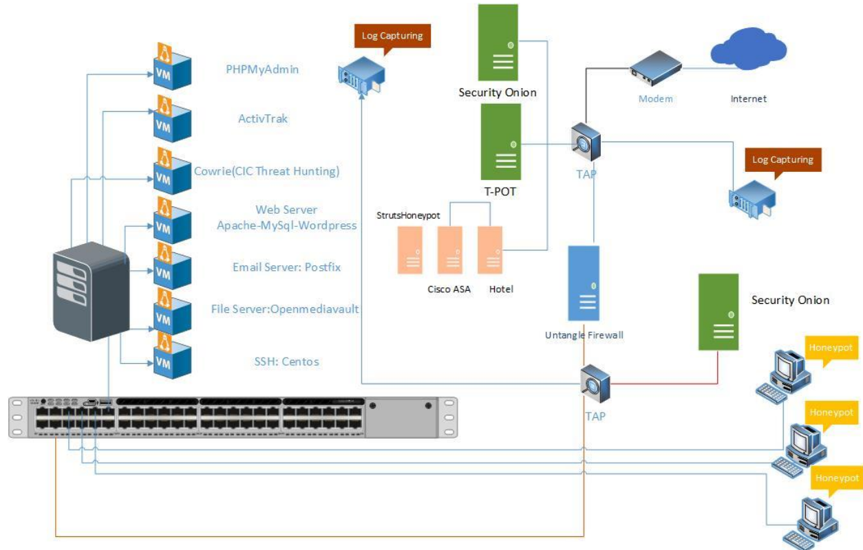
Figure2: Network Diagram
